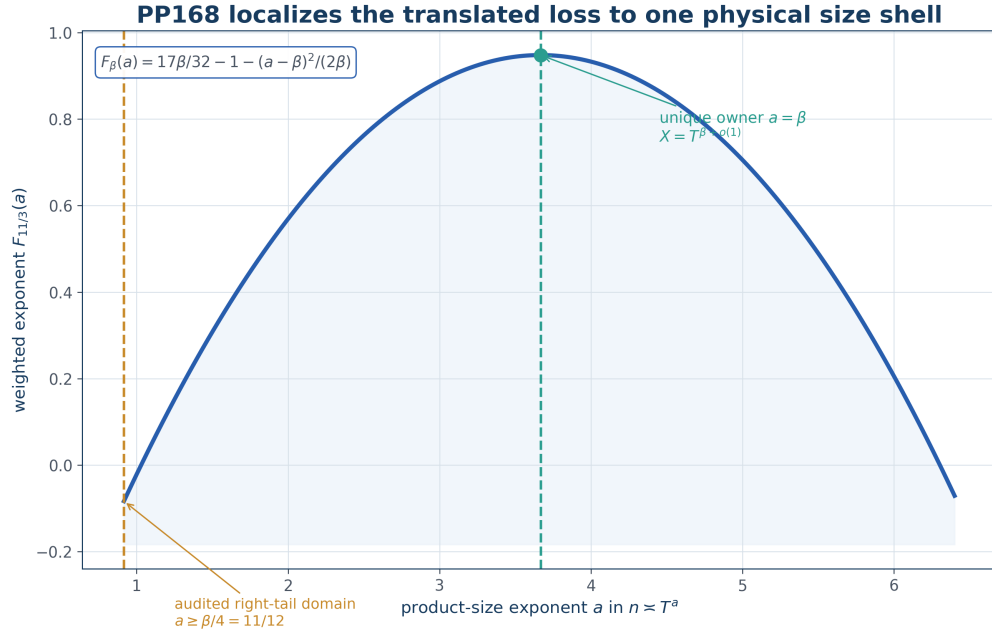
Figure 51: The weighted exponent is a strict parabola whose maximum sits on the single shell X = T^\beta .
