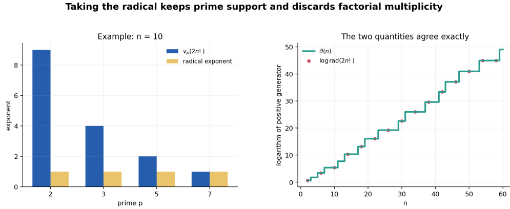
Figure 3: The ideal radical preserves prime support while discarding factorial multiplicity.
