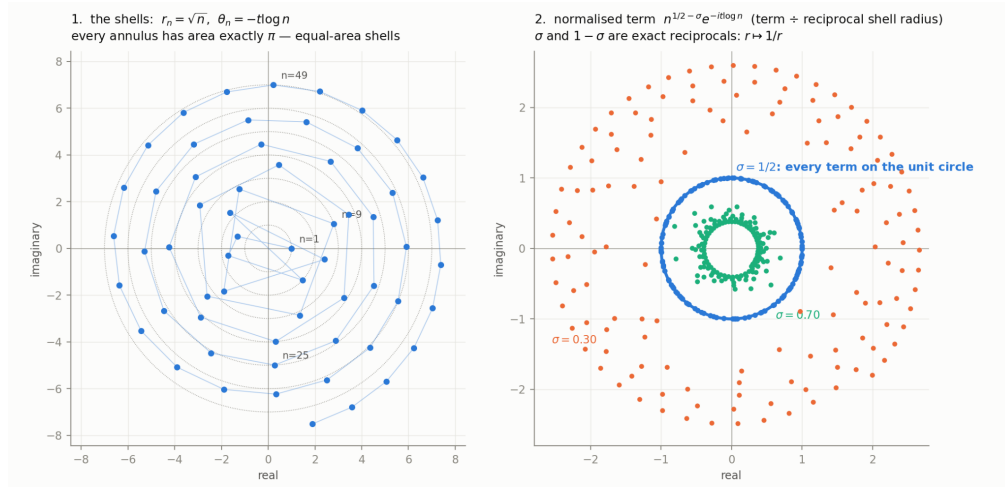
Figure 12: Equal-area polar shells and the 1/\sqrt{n} normalization. The angular laws differ, but every complex phase must retain its conjugate partner.
