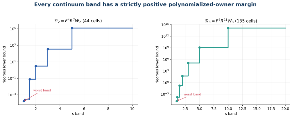
Figure 32: The finite W_2 and W_3 continuum certificates have positive lower bounds on every band; the two panels show different polynomialized expressions and should not be compared in absolute scale.
