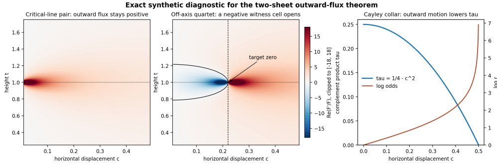
Figure 28: Synthetic critical-line and off-axis flux fields, together with the Cayley collar coordinate.
