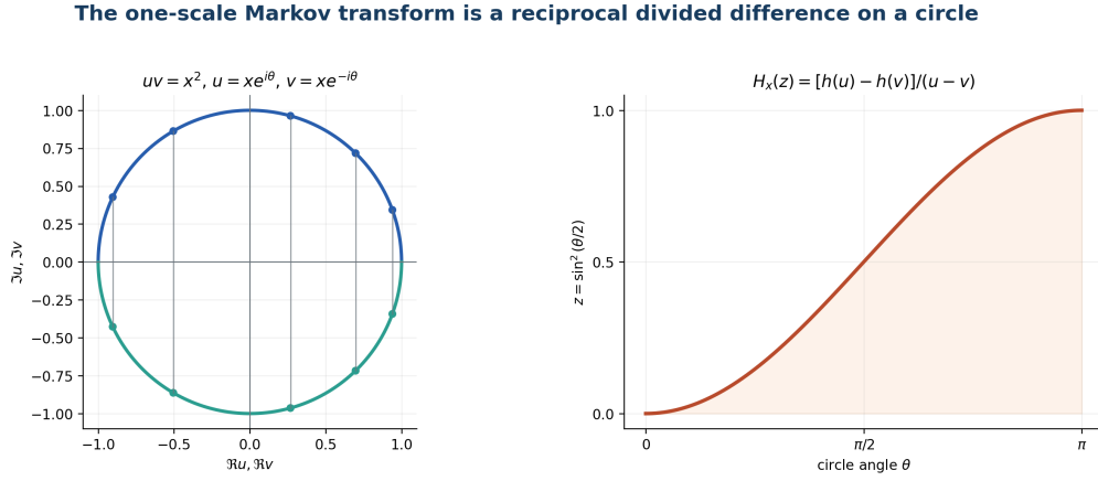
Figure 41: The reciprocal pair u, v runs on a circle, and the Markov parameter is z = \sin^2(\theta/2) .
