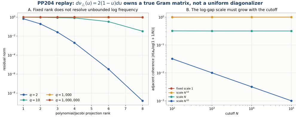
Figure 60: Projection and scale diagnostics for the Beta-logarithm model. Each curve is finite and replayed; the plotted trend is a firewall, not an asymptotic proof beyond the stated theorem.
