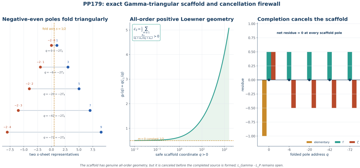
Figure 17: The Gamma triangular scaffold is positive before completion; completion cancels its apparent triangular poles.
